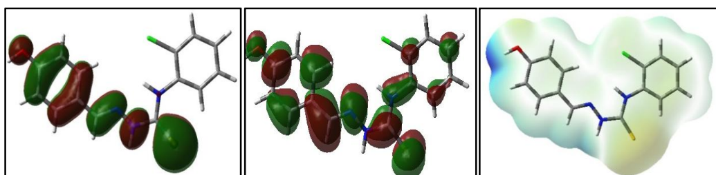
Molecule 11-HOMO
