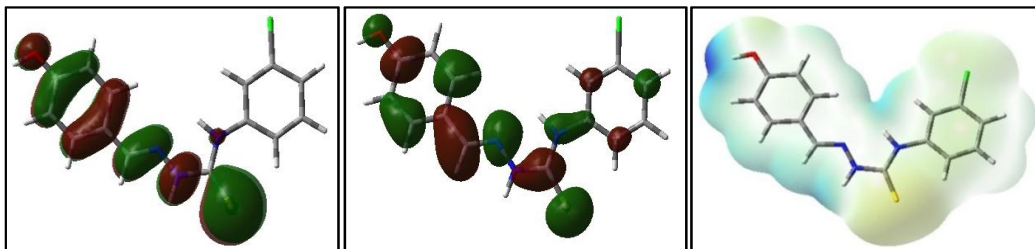
Molecule 12-HOMO
