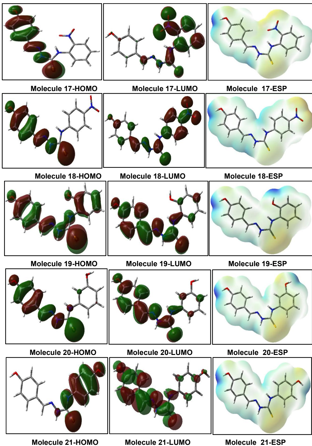
Fig. 1. HOMO, LUMO & ESP of the active molecules
