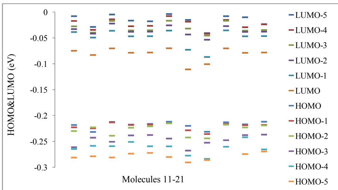
Fig. 2-b. HOMO & LUMO of molecules 11-21 at B3LYP/6-311G (d,p)
