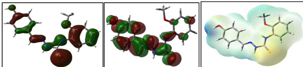
Molecule 16-HOMO
