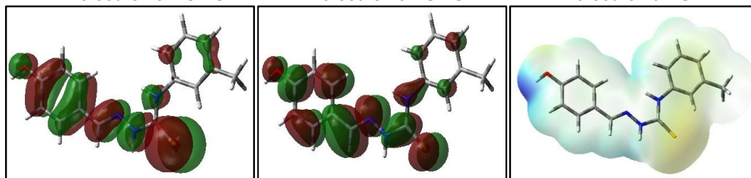
Molecule 14-HOMO
