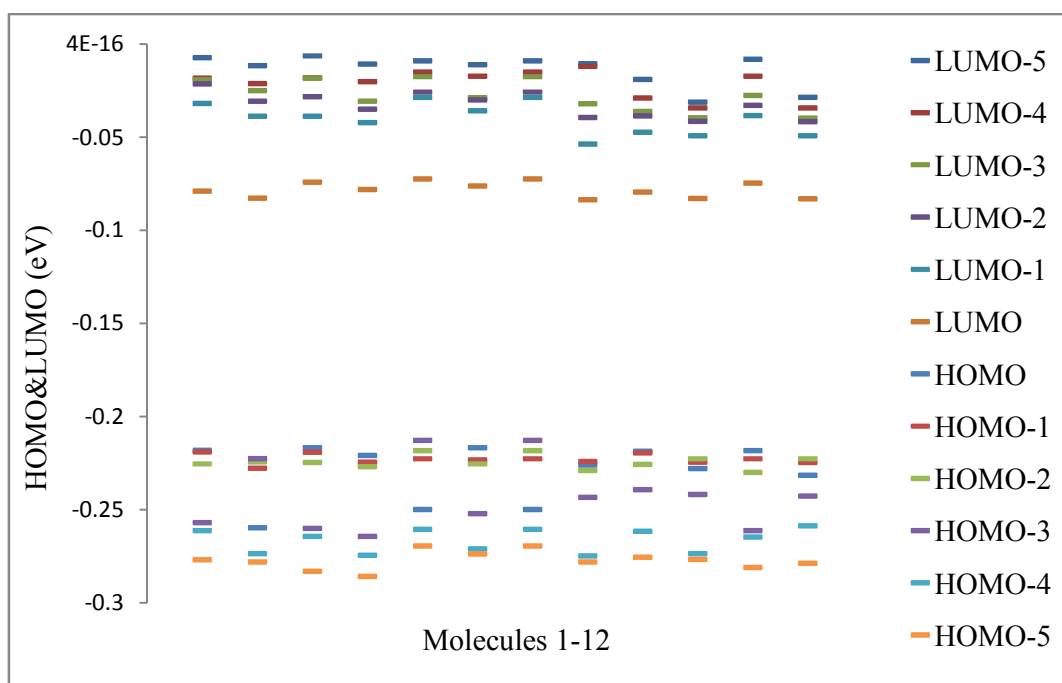
Fig. 2-a. HOMO & LUMO molecules 1-12 at B3LYP/6-311G(d,p)
