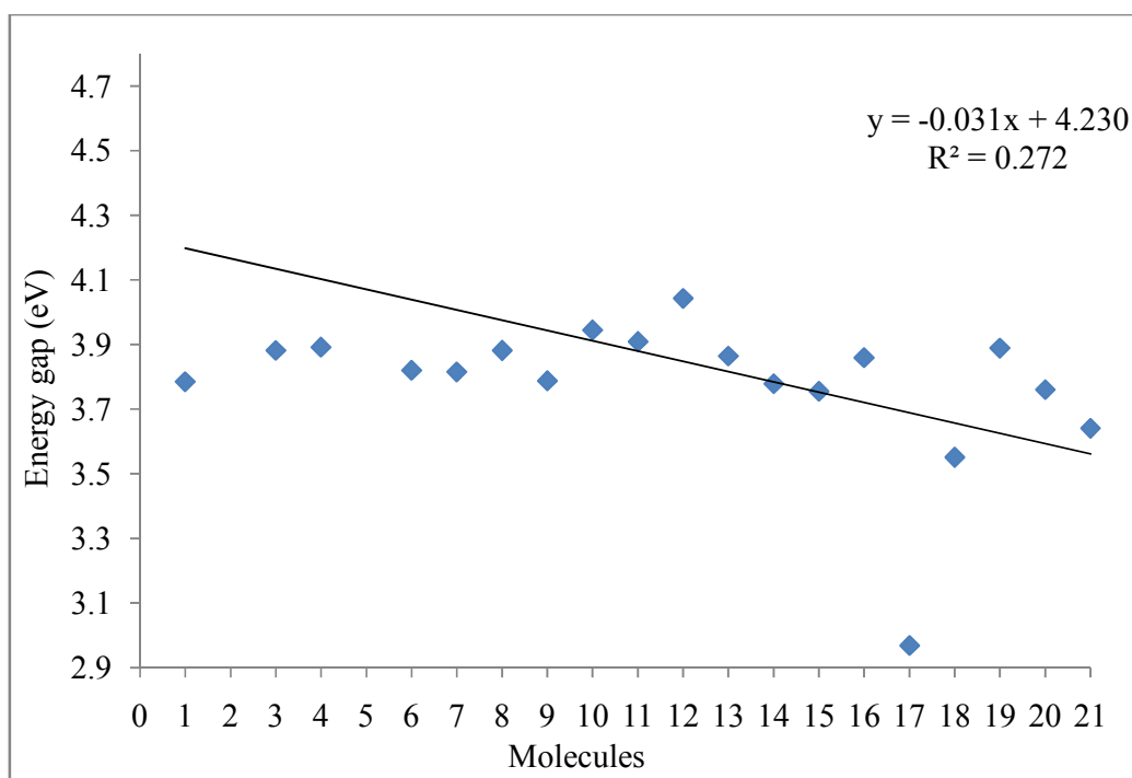
Fig. 3. The energy gap relation to the molecules
